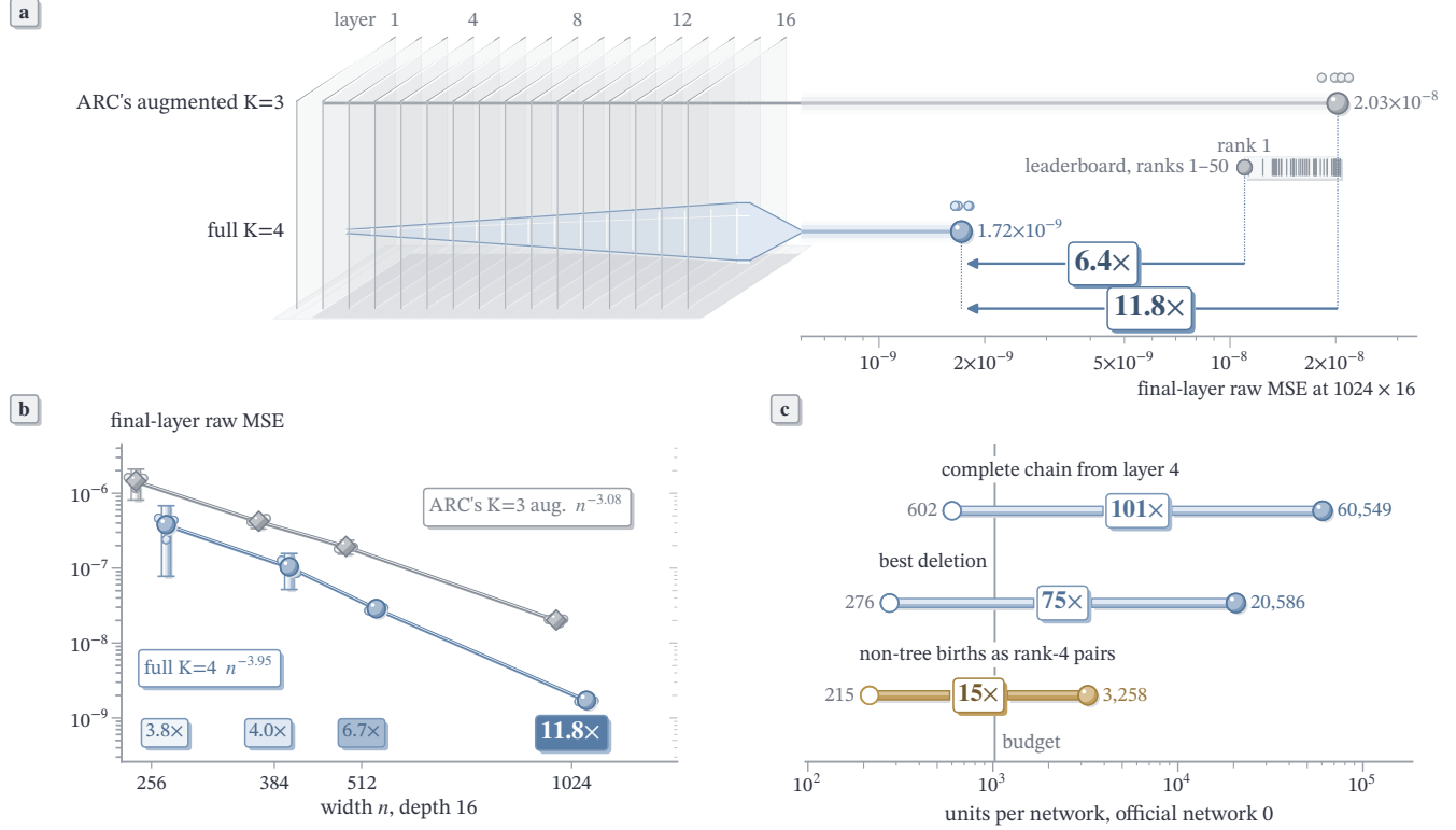
Figure 0: Exact unaugmented K=4 at 1024 \times 16 ends 11.8\times below augmented K=3 on all five official networks and 6.4\times below the lowest raw error on the leaderboard, its error falling as n^{-3.95} . (a) The 16 layers of the five official networks as the glass plates of Figure 3; the K=4 state's width counts its live source groups, and each beam ends at its final-layer raw MSE on one log ruler (large disc the mean, small discs the networks). Ticks: each entry ranked 1–50 on the official leaderboard (18 October), on its 50 networks. (b) Small discs networks, large marks means, tubes 95% t intervals. (c) Official network 0 from layer 4: counted units (disc), units at which each configuration ties our scored chain (ring).
