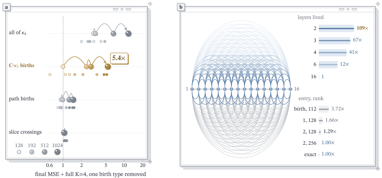
Figure 2: Carried births, not local accuracy, hold the gain: removing C\cdot\kappa_3 births costs 5.4\times on official networks 0–1 at width 1024, the largest single removal, and 4.7\text{--}5.2\times on three networks frozen before running; letting every source live only two layers costs 109\times . (a) One row per birth type removed from full K=4 , final \text{MSE} \div \text{full } K=4 : beads are widths 128, 192, 512 and 1024, lighter to deeper and joined in that order; small dots are single networks frozen before running (at 128 and 192, and networks 5, 6 and 7 at 1024); the dashed line is no change (Table 3). (b) The K=4 state of official network 0 at width 1024, drawn as its reads: each arc joins a source's birth layer to a later layer that reads it, shaded by age. Above the axis, the ladder gives final MSE as a multiple of keeping every source for all 16 layers, when each lives 2, 3, 4 or 6; below, gray arcs are the reads made after a source enters a shared basis two transports after birth, and the ladder gives final \text{MSE} \div \text{exact} for each entry age and basis rank, on the same log scale.
