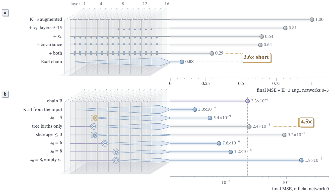
Figure 3: Memoryless patches stall where the carried chain does not: on official networks 0–3, augmented K=3 handed the K=4 chain’s own covariance and \kappa_4 at every layer reaches 0.29 of its error, the K=4 chain 0.08, 3.6 \times lower; started at layer 4 from chain B, K=4 reaches 5.42e-9, and without its non-tree births it is 4.5 \times worse. Each chain runs left to right through its 16 layers, drawn as glass plates: gray is augmented K=3, iris chain B, blue the K=4 state, whose width counts its live source groups (hatched: tree births only); a ring marks where the K=4 state starts, the open ring from an empty fourth cumulant, and each beam leaving layer 16 reads out the final MSE. (a) Official networks 0–3, as a ratio to augmented K=3; squares and diamonds mark the layers at which the exact covariance and \kappa_4 are handed in. (b) Official network 0; the dashed line is chain B alone, and the slice-age row caps how long the slice groups of the tree-only run live.
