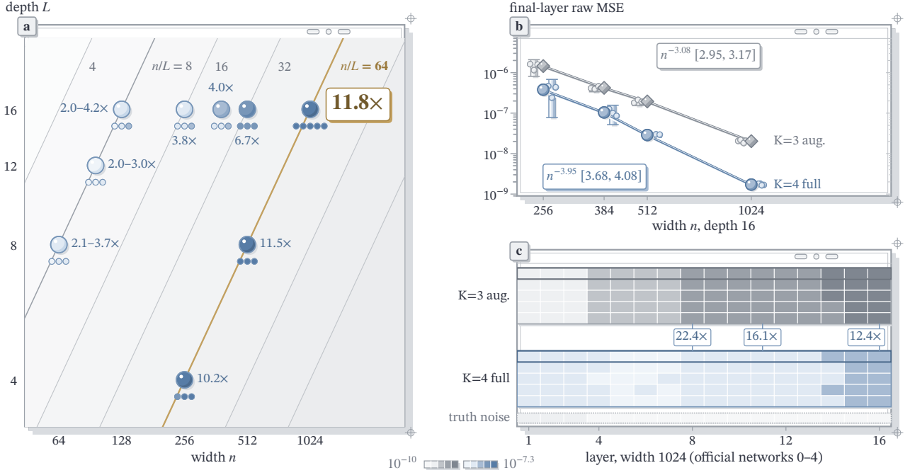
Figure 1: Exact unaugmented K=4 scales as n^{-3.95} against augmented K=3’s n^{-3.08} and cuts final-layer MSE 11.8 \times below it at 1024 \times 16 on all five official networks; the gain follows n/L , 10.2–11.8 \times for all three shapes at n/L = 64 and 2.0–4.2 \times on the nine networks at n/L = 8 , the ratio at which F29 found augmented K=4 behind. (a) Every measured shape at its width and depth; the diagonals are lines of constant n/L , the bands between them deeper as n/L grows. A station’s shade and label give K=3 aug. \div K=4 full as a ratio of mean errors (at n/L = 8 the range over its three networks), the dots beneath it the ratio on each network. (b) Raw final-layer MSE against width at depth 16: small discs are single networks (three per width, the five official networks at 1024), large marks their means, tubes 95% t intervals, chips the fitted exponents with 95% network-resample intervals. (c) Per-layer MSE of the five official networks at width 1024, one cell per network and layer, network 0 on top and outlined; chips are the noise-removed ratio at layers 8, 11 and 16, the bottom strip the truth’s sampling noise. Tables 2 and 2b (Appendix A.8) list every value.
