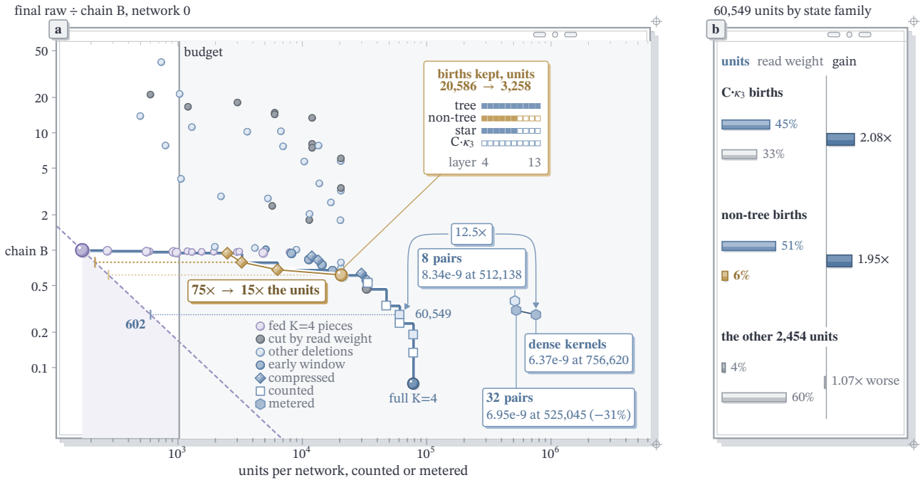
Figure 5: One compute–error frontier on official network 0, inside the budget and beyond it: deleting state stalls at 75 times the units its accuracy may cost (0.615× of chain B’s error at 20,586 units), rank-4 non-tree pairs cut that to 15 times (0.788× at 3,258), and the metered whole chain falls from 756,620 units with dense kernels to 525,045 with 32 matrix pairs at 6.95e-9. (a) Every measured configuration on official network 0, final raw over chain B’s against counted units; the stair is the lower envelope over both batches, the best raw at no more units. The dashed diagonal is chain B’s score, so a point’s horizontal distance to it is the factor by which its units exceed what its accuracy may cost; past the budget line a network scores as all zeros. Gold: the 20,586-unit rule and, along the gold line, the same births with non-tree pairs of rank 16, 4 and 1, the dotted lines ending at their ties (Table 11); blue diamonds hold both families as pairs. Squares are counted (Table 7a); hexagons are metered end to end by floscope (Table 12) and joined as the metered line, each capsule naming its run: the compressed chain from layer 4 with dense (2,1,1) kernels, 6.37e-9 at 756,620 units, and the same chain with its (2,1,1) births as 32 matrix pairs, 6.95e-9 at 525,045 (31% fewer units), and as 8 pairs, 8.34e-9 at 512,138. The arc joins the counted chain from layer 4 (60,549 units) and the dense metered run at one raw: the meter reads 12.5× the count. Chain B’s disc and the fed K=4 pieces give the frontier’s scored side. The card shows which births the rule keeps, layer by layer. (b) The layer-4 column of Table 7a by family: share of the units, share of the first-order read weight and the gain, final error without the family over with it; for the other 2,454 units, the tree slices alone against chain B. Tables 9 and 10 list the values.
